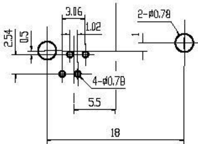
PCB Mounting Layout.
